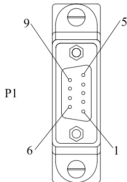
DB9P(F) PLASTIC:BLUE
