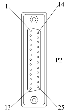
DB25P(F) PLASTIC:BLUE
